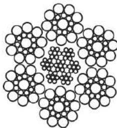
Conventional Rope
